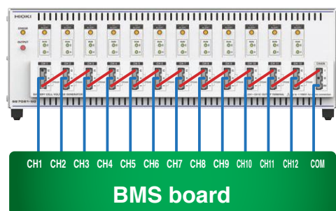
12 channel connection example
