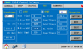
High Voltage Ride Through Setting
