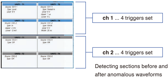
Setting Screen with Easy-to-Understand Trigger System Chart
