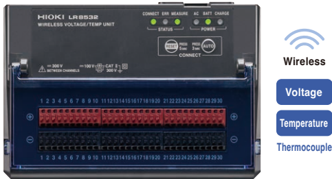
WIRELESS VOLTAGE/TEMP UNIT LR8532
