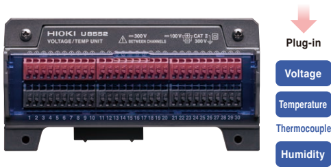
VOLTAGE/TEMP UNIT U8552
