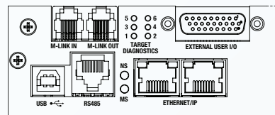
Rear communication interfaces with EtherNet/IP (+EIP) option.
